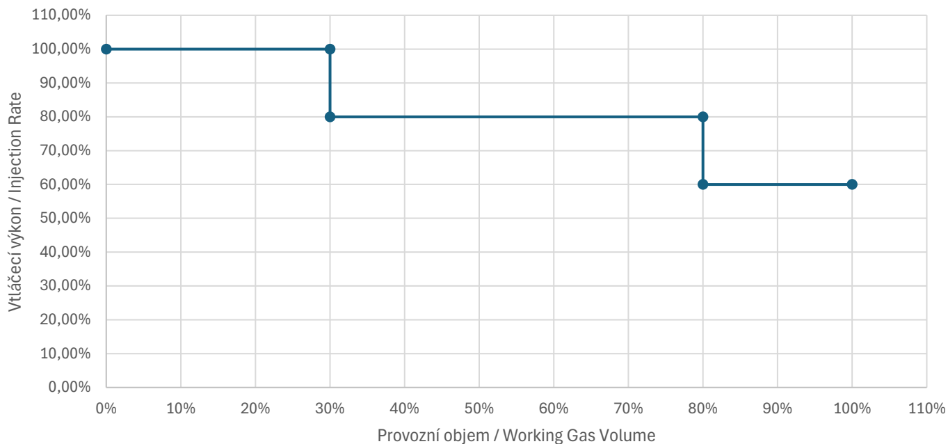
Vtláčečí křivka / Injection Curve
